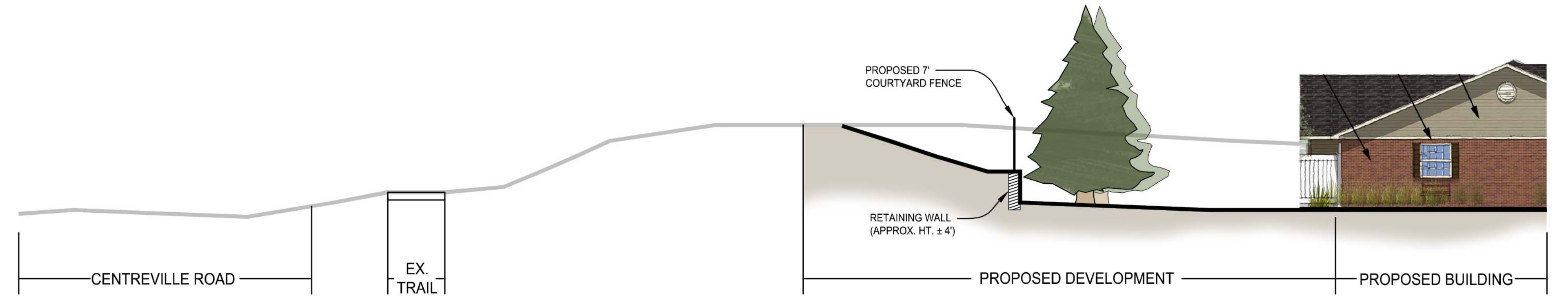
Cross Section A-A'
