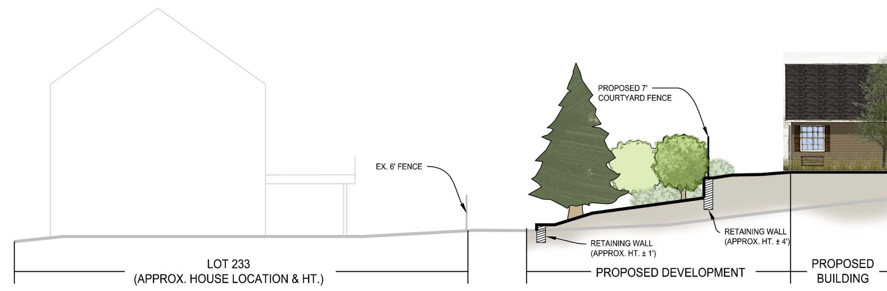
Cross Section C-C'
